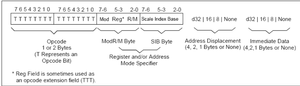
Figure 7: Pentium General Instruction Format
