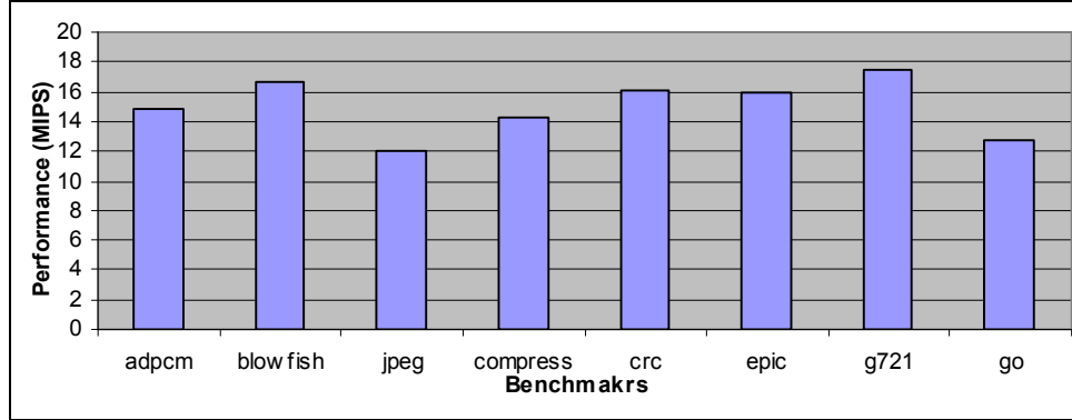
Figure 11: Simulation Results of ARM7 processor
